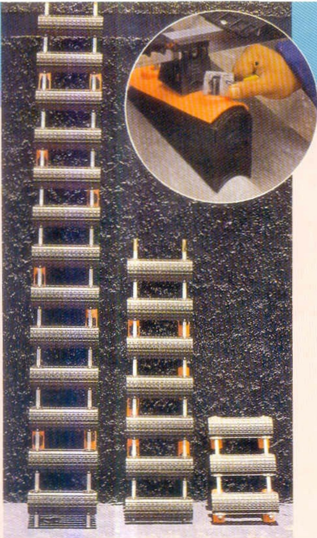
Inset : Elevating pads used on excessively inclined roofs and Quick-action clamps used on bolts coated with tar or corroded
